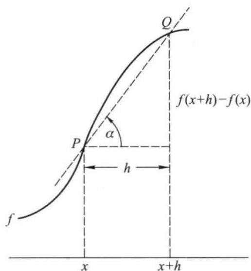
Fig.2-8-1 Geometric interpretation of the difference quotient as the tangent of an angle
