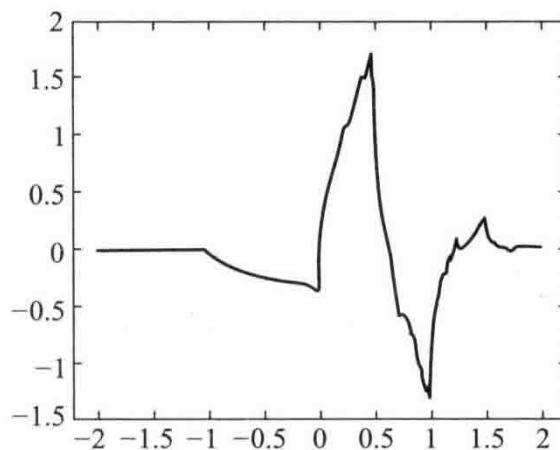
Fig. 3-6-4 Graph of Daubechies wavelet
