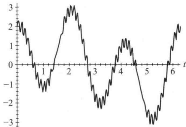
Fig. 3-6-1 Plot of f(t) = \sin(t) + 2\cos(3t) + 0.3\sin(50t)
