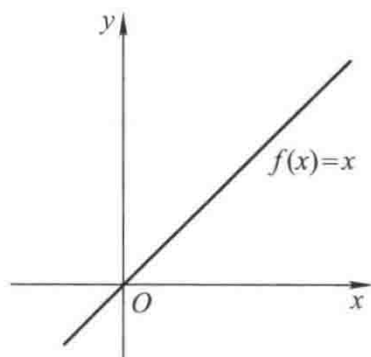
Fig.2-6-2 Graph of the identity function f(x) = x
