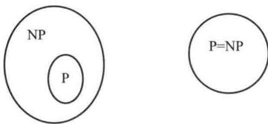
Fig. 3-5-2 One of these two possibilities is correct.
