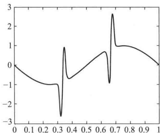
Fig. 3-6-3 Graph of a signal with isolated noise
