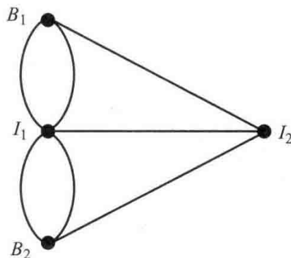
Fig.3-4-7 The graph of the bridges of Königsberg problem.
