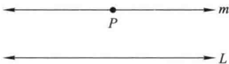
Fig. 3-3-1 Lines L and m are parallel.
