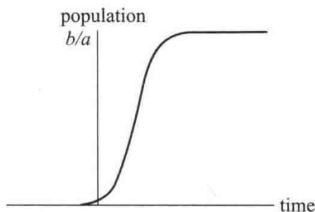
Fig. 3-4-5 A typical logistic curve.
