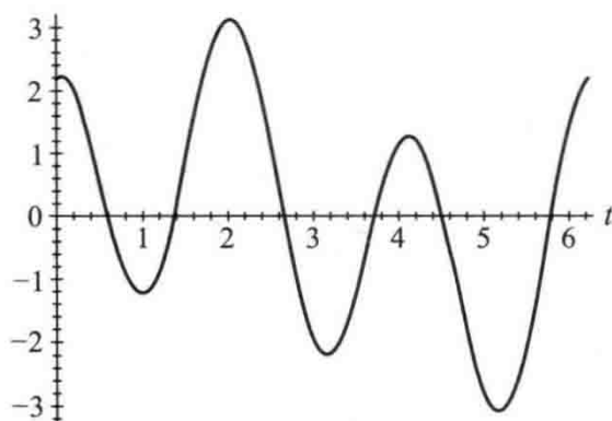
Fig. 3-6-2 Plot of f(t) = \sin(t) + 2\cos(3t)
