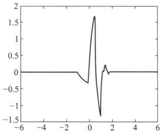
Fig. 3-6-5 High-frequency Daubechies wavelet
