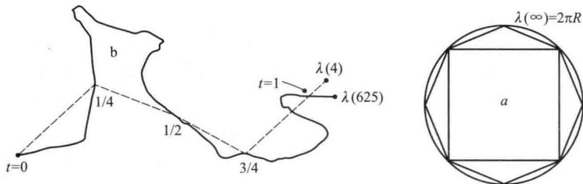
Fig. 3-6-6 Approximation to a curve by steps of length \eta , for p=4 and p=625 .
