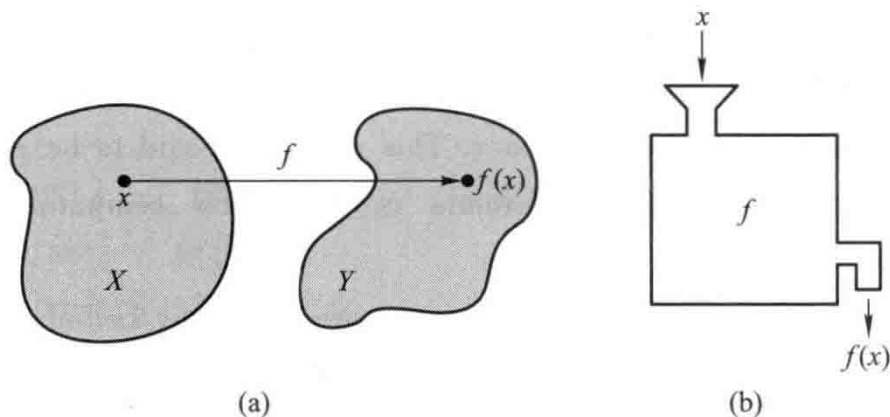
Fig.2-6-1 Schematic representations of the function idea
