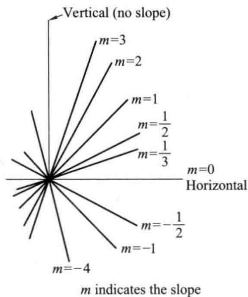
Fig.2-8-2 Lines of various slopes
