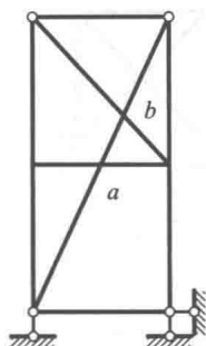
题 2-9 ( a, b 处非结点)
